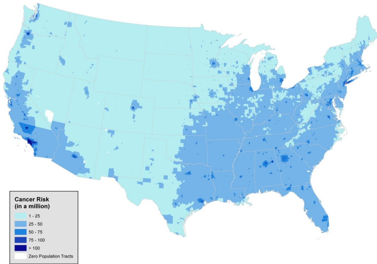
Figure 4-4. Estimated Census Tract Carcinogenic Risk from HAP exposure from outdoor sources (2005 NATA)
