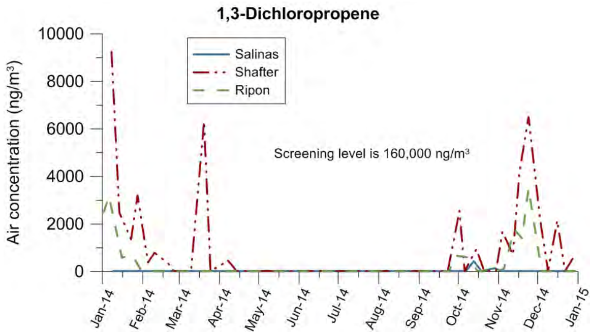
Figure 7. Highest 24-hour (acute) concentrations detected for the aggregate of cis - and trans -1,3-dichloropropene at each of three sampling locations.
